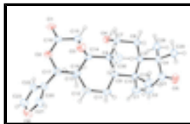
Fig. 1. The molecular structure of the title compound showing 30% probability displacement ellipsoids and the atom-numbering scheme in one independent molecule.
